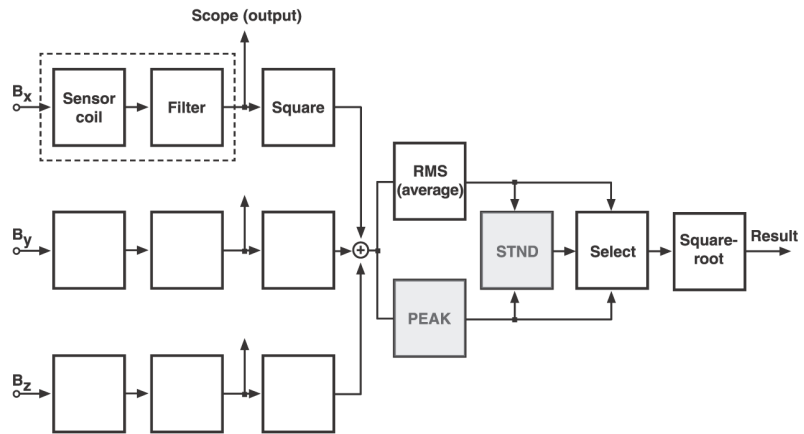
Fig. 2: Diagram of the reference method according to EN 50366. Scope (oscilloscope output), PEAK (peak value detector) and STND (standard) are special features of the Narda Safety Test Solutions ELT-400 test set, which can also evaluate fields on the basis of other standards.
