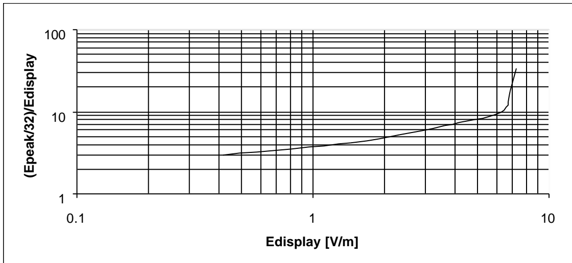
Fig. 9 "Dynamic" corrective curve (probe 1) for the air surveillance radar
