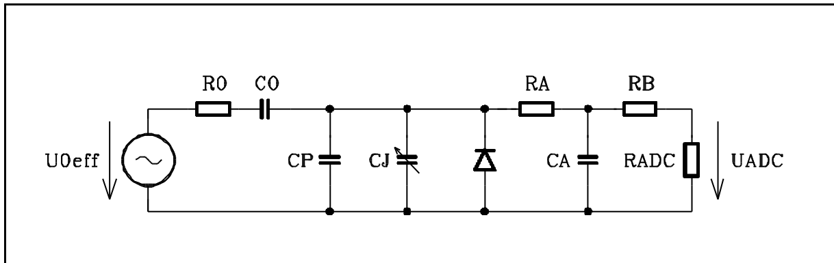
Fig. 2 Equivalent circuit of W&G EMR-300 for a transient analysis
