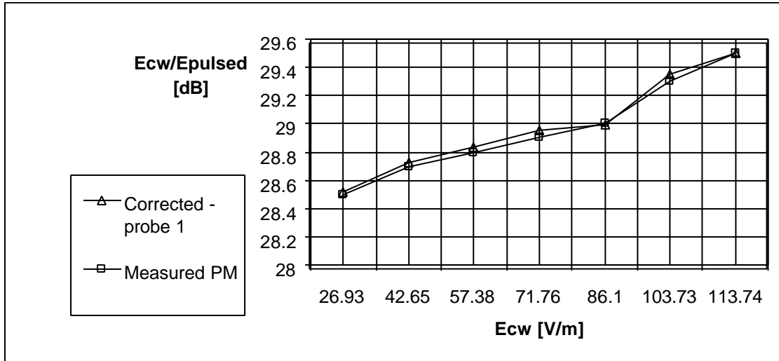
Fig. 8a Ratio of continuous wave and pulsed field displayed by the meter and corrected according to the simulated curves (Fig. 6) and the measured values with power meter for the probe 1
