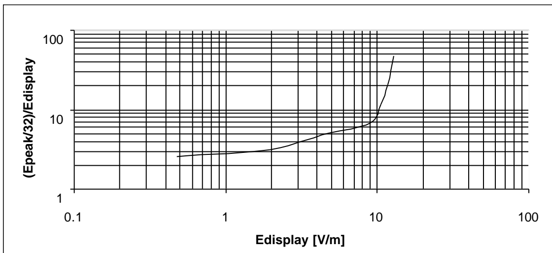
Fig. 10 "Dynamic" corrective curve (probe 2) for the air surveillance radar
