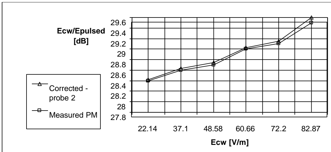
Fig. 8b Ratio of continuous wave and pulsed field displayed by the meter and corrected according to the simulated curve (Fig. 7) and the measured values with power meter for the probe 2
