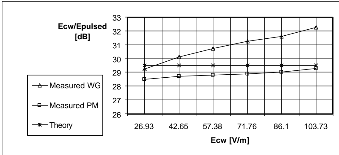
Fig. 4 Ratio of continuous wave and pulsed field displayed by the meter, by the power meter and theoretically calculated values for probe 1
