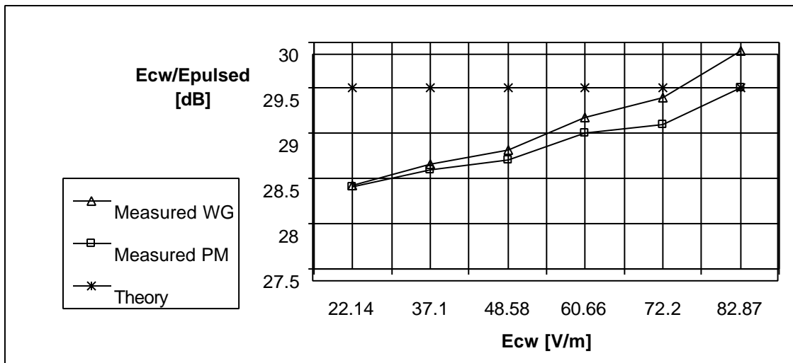
Fig. 5 Ratio of continuous wave and pulsed field displayed by the meter, by the power meter and theoretically calculated values for probe 2
