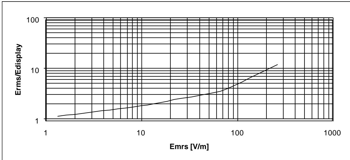
Fig. 6 "Static" correction curve for probe 1 (simulation)
