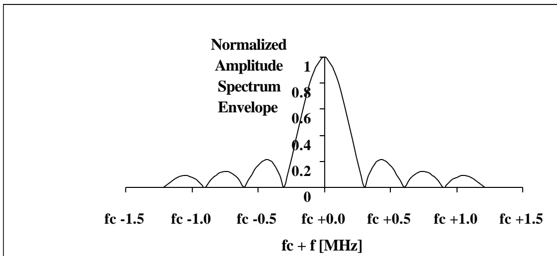
Fig. 1 Frequency spectrum of a radar pulse train
