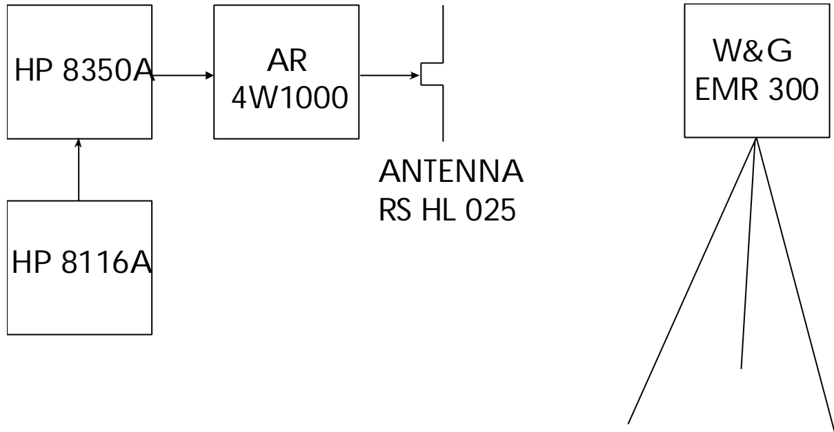
Fig. 3 The measurement set-up
