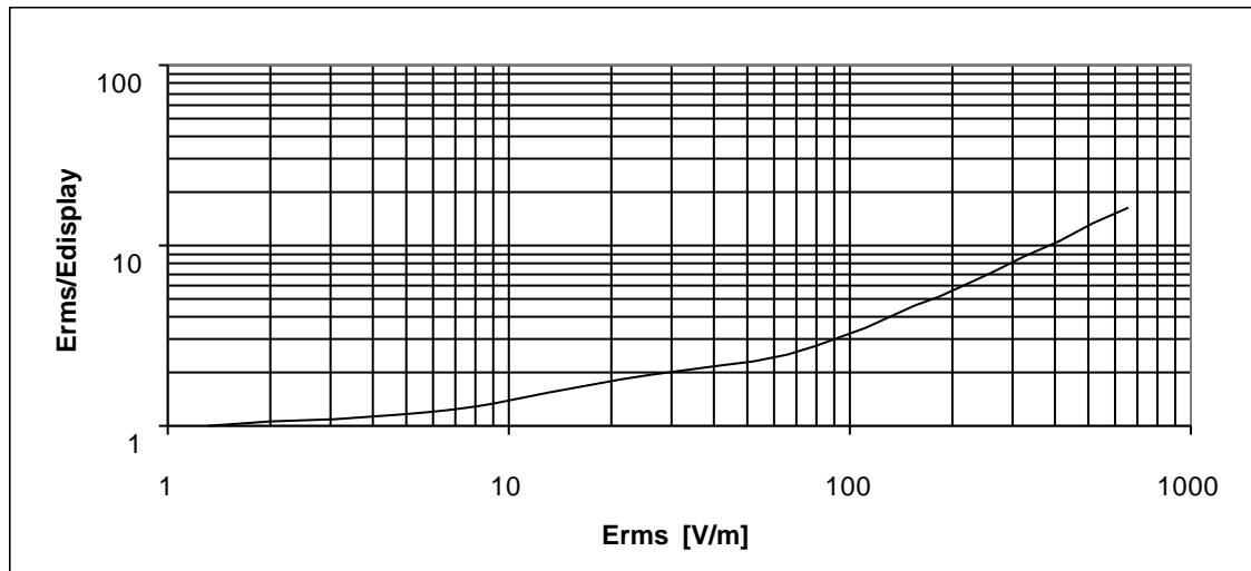
Fig. 7 "Static" correction curve for probe 2 (simulation)
